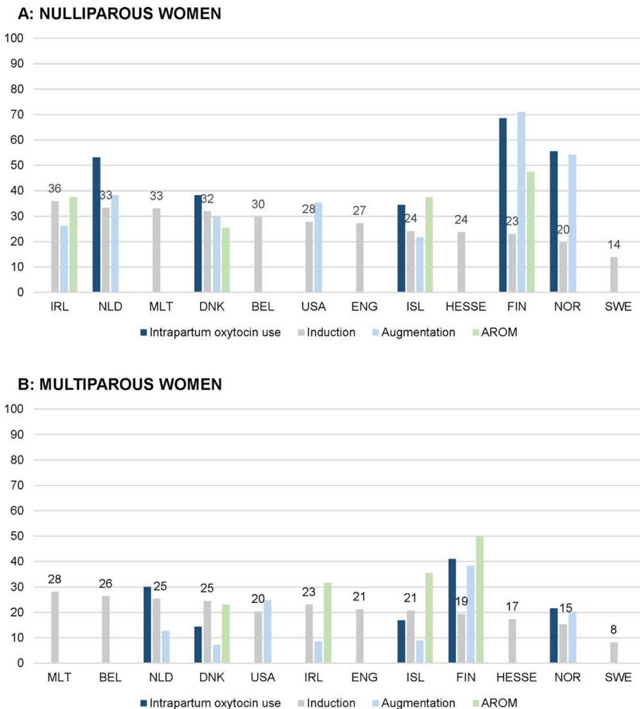
Fig 3. Inter-country variation of interventions to stimulate uterine contractions in 2013 (%). (A) Nulliparous women. (B) Multiparous women. AROM, artificial rupture of membranes; BEL, Belgium; CHL, Chile; DNK, Denmark; ENG, England; FIN, Finland; HESSE, the state of Hesse (Germany); IRL, Ireland; ISL, Iceland; MLT, Malta; NLD, the Netherlands; NOR, Norway; SWE, Sweden; USA, United States of America.
