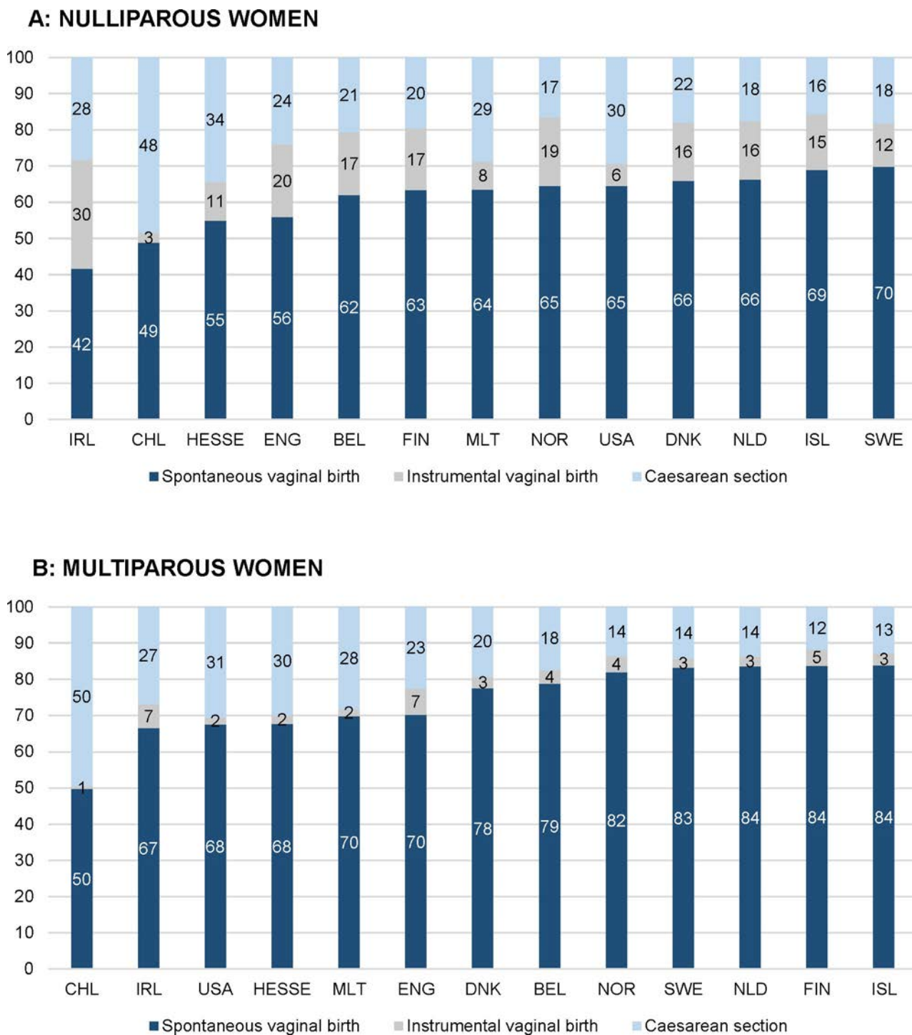
Fig 2. Inter-country variation of mode of birth in 2013 (%). (A) Nulliparous women. (B) Multiparous women. BEL, Belgium; CHL, Chile; DNK, Denmark; ENG, England; FIN, Finland; HESSE, the state of Hesse (Germany); IRL, Ireland; ISL, Iceland; MLT, Malta; NLD, the Netherlands; NOR, Norway; SWE, Sweden; USA, United States of America.
